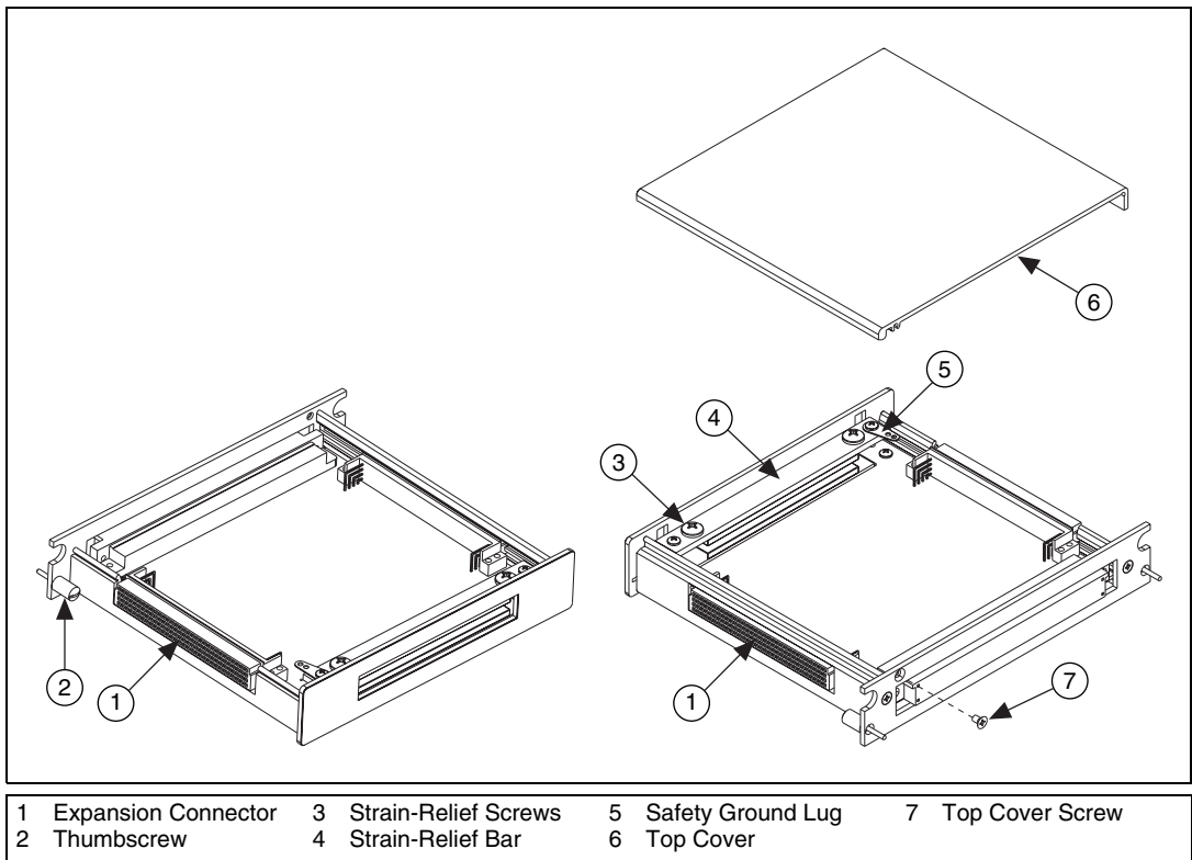
Figure 1. SCXI-1334 Parts Locator Diagram
